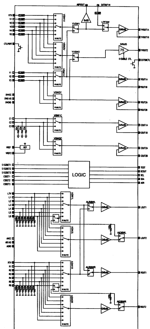
Fig-2 BLOCK DIAGRAM
